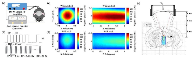
Illustration of ultrasound stimulation system. Credit: NIU Lili
