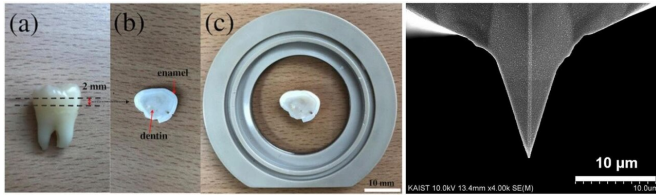
Tooth sample preparation process for atomic force microscopy (a, b, c), and an atomic force microscopy probe image (right). Credit: Professor Seungbum Hong, KAIST
