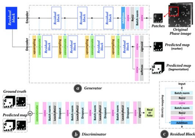
Overview diagram of deep learning algorithm with proposed two-step structure for erythrocyte holography image segmentation and automatic classification. Credit: DGIST (Daegu Gyeongbuk Institute of Science and Technology)
